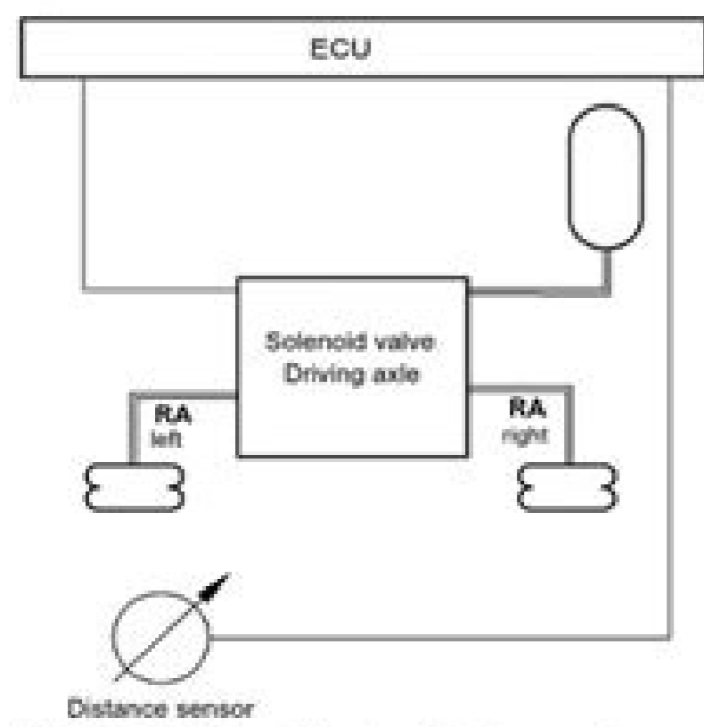
Abb. 13 Control for vehicles with partial air suspension
