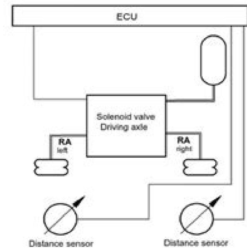
2-point control
